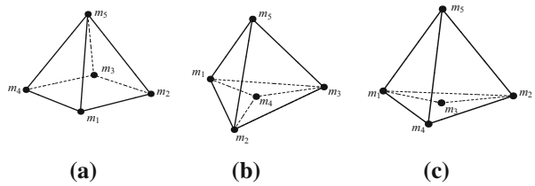
Fig. 5 Central configurations of the spatial (4 + 1) -body problem with four equal masses at the vertices of a planar central configuration. a Class P_S , b class P_{et} , c class P_{it}
