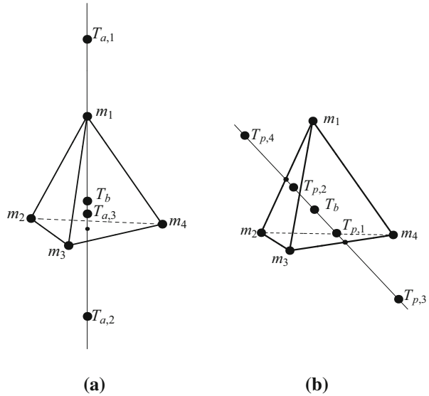
Fig. 3 Central configurations of the spatial (4 + 1) -body problem with four equal masses at the vertices of a regular tetrahedron. a Axis type symmetry, b planar type symmetry
