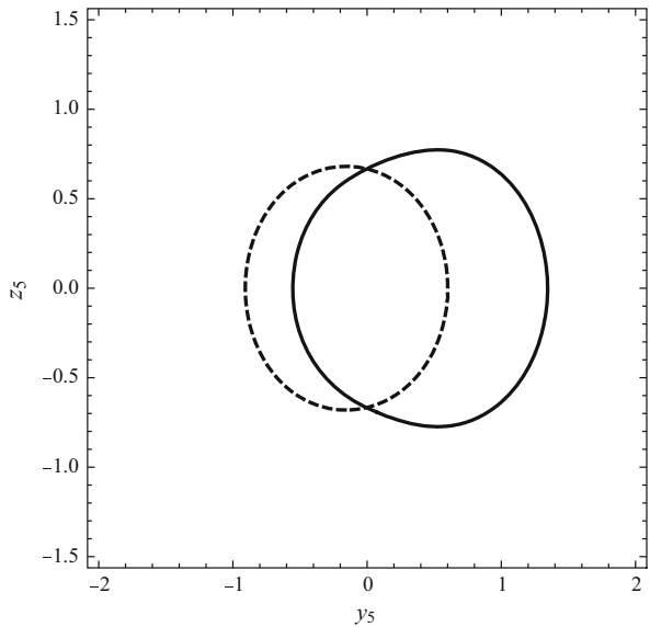
Fig. 4 The level curves \bar{f}_3(y_5, z_5) = 0 (continuous line) and \bar{f}_4(y_5, z_5) = 0 (dashed line)
