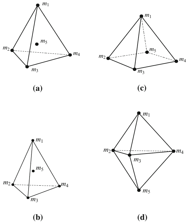
Fig. 2 Central configurations of the spatial 5-body problem with equal masses. a Class K_1 , b class K_3 , c class K_2 , d class K_4
