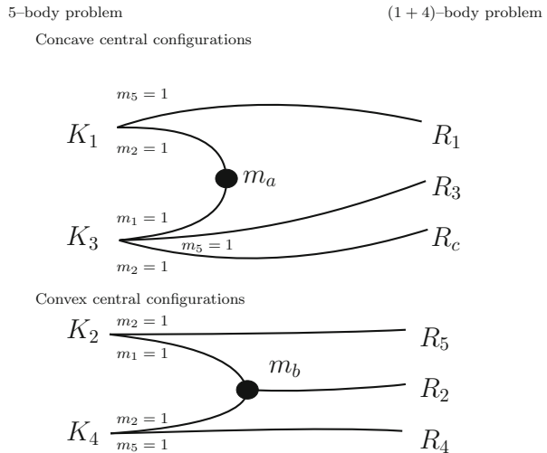
Fig. 8 Connections between the classes of central configurations of the (5)-body problem with equal masses and the ones of the spatial (1 + 4)-body problem with equal infinitesimal masses. Each line corresponds to a different family of central configurations of the 5-body problem with 4 equal masses. The black dots represent mass values where degenerate central configurations occur
