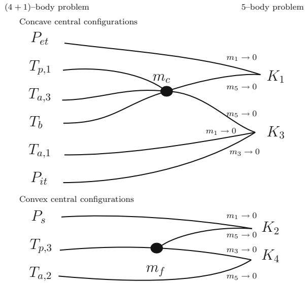
Fig. 7 Connections between the classes of central configurations of the (4 + 1) -body problem with 4 equal masses and the ones of the spatial 5-body problem with equal masses. Each line corresponds to a different family of central configurations of the 5-body problem with 4 equal masses. The black dots represent mass values where degenerate central configurations occur
