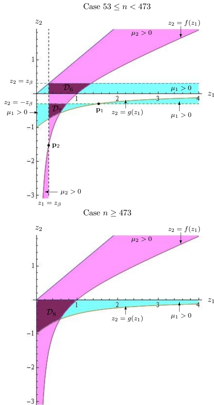
FIGURE 3. The regions delimited by the curves z_2 = g(z_1) , z_2 = 0 , z_2 = \pm z_\beta , z_2 = f(z_1) , and z_1 = z_\beta restricted to \{(z_1, z_2) \in \mathbb{R}^2 : z_1 > 0, z_1 > z_2\} , and the sign of \mu_1 and \mu_2 on each region for n \geq 53 .
