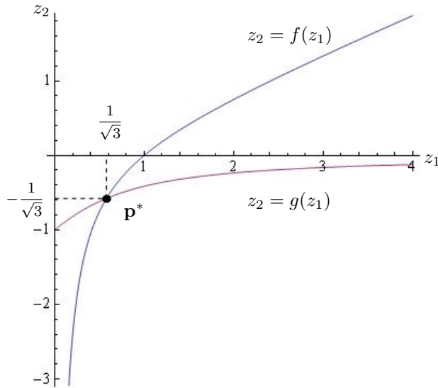
FIGURE 1. The plot of the curves z_2 = f(z_1) and z_2 = g(z_1) .
