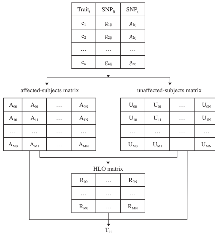
Figure 4 Decomposition of the different steps of the computation of T_{ij} . c_a is 1 (0) if the a^{\text{th}} subject is a case (control) for the i^{\text{th}} permutation of the trait. g_{alj} and g_{arlj} are 0, 1 or 2 depending on the genotype of the a^{\text{th}} subject for the j^{\text{th}} pair. A_{mn} and U_{mn} are respectively the number of affected/unaffected subjects, whose genotype g_{kl} = m and g_{kr} = n . R_{mn} is either "H" if the subjects whose genotype is m for SNP_{lj} and n for SNP_{rlj} have a high statistical risk of disease, "L" if they have a low statistical risk and "O" if there is no statistical evidence.
